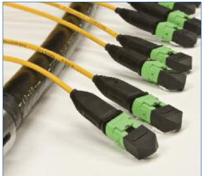
Ruggedized Zone Enclosure with Preterminated MTP End | Photo LAN1301
